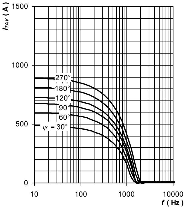
Fig. 33 Average on-state current vs. frequency, trapezoid waveform, T_C = 90^\circ\text{C} , di_T/dt = \pm 500\text{ A}/\mu\text{s} , V_R = 100\text{ V}
