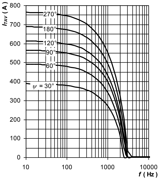
Fig. 21 Average on-state current vs. frequency, trapezoid waveform, T_C = 70\text{ }^\circ\text{C} , di_T/dt = \pm 100\text{ A}/\mu\text{s} , V_R = 100\text{ V}
