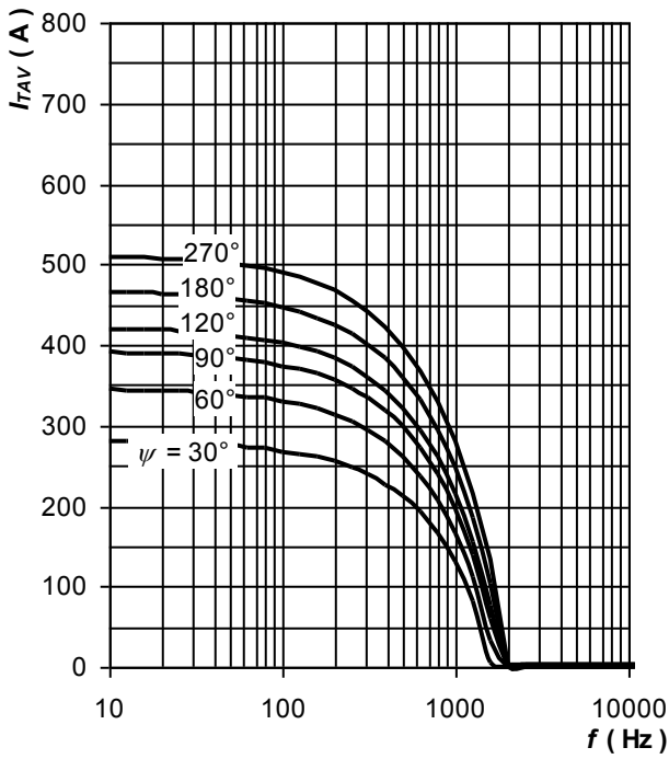
Fig. 29 Average on-state current vs. frequency, trapezoid waveform, T_C = 90\text{ }^\circ\text{C} , di_T/dt = \pm 100\text{ A}/\mu\text{s} , V_R = 100\text{ V}
