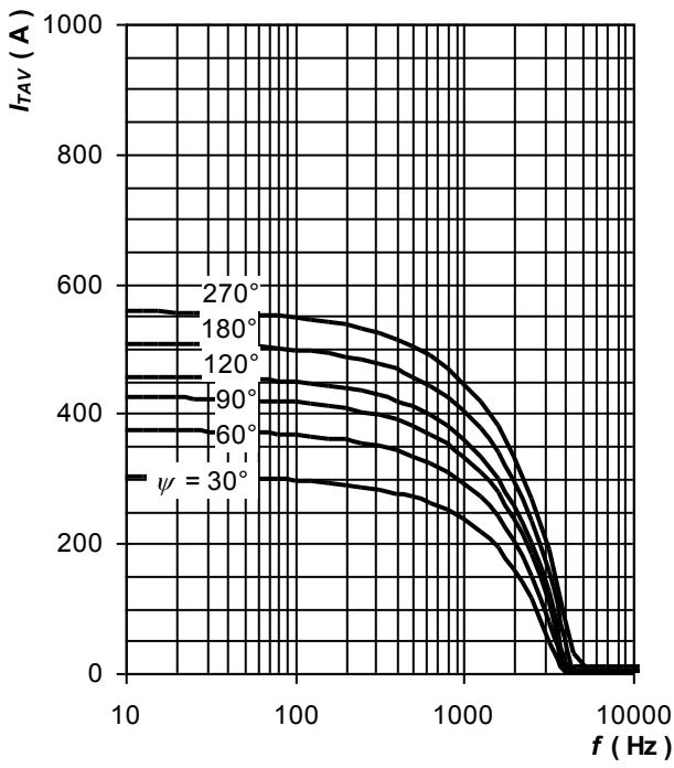
Fig. 31 Average on-state current vs. frequency, trapezoid waveform, T_C = 90\text{ }^\circ\text{C} , di_T/dt = \pm 100\text{ A}/\mu\text{s} , V_R = 2/3 V_{DRM}
