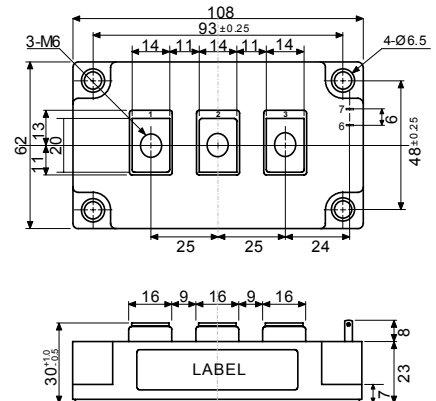
PRFMB600E6C
